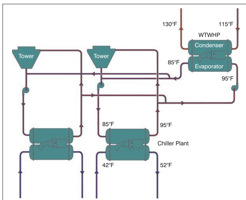
Figure 4: Tower water as heat source.
