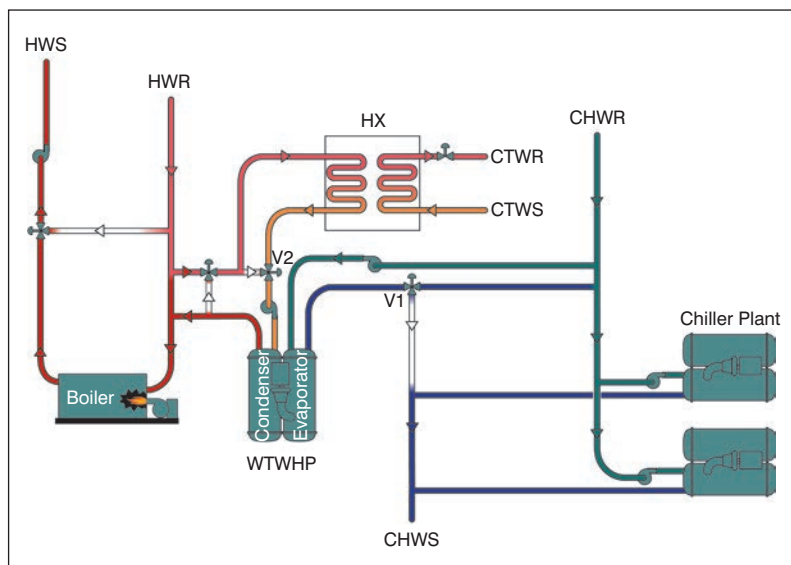
Figure 7: Hybrid side-stream/parallel system, operating in side-stream arrangement.
