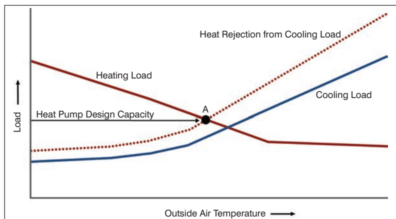
Figure 1: Selection point for simultaneous heating-and-cooling heat pump.
