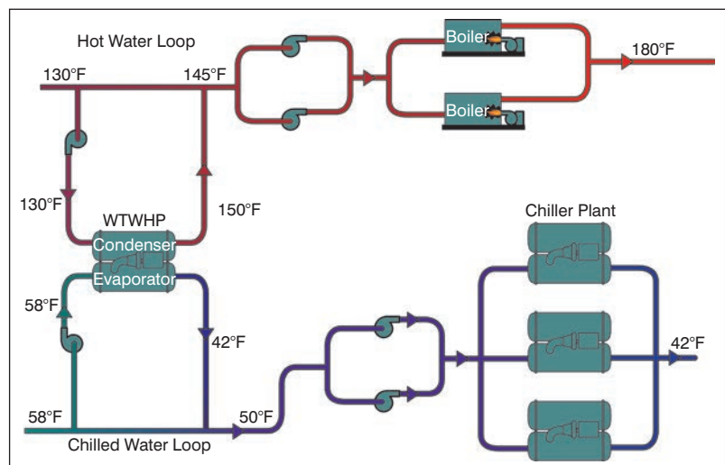
Figure 6: Side-stream arrangement.
