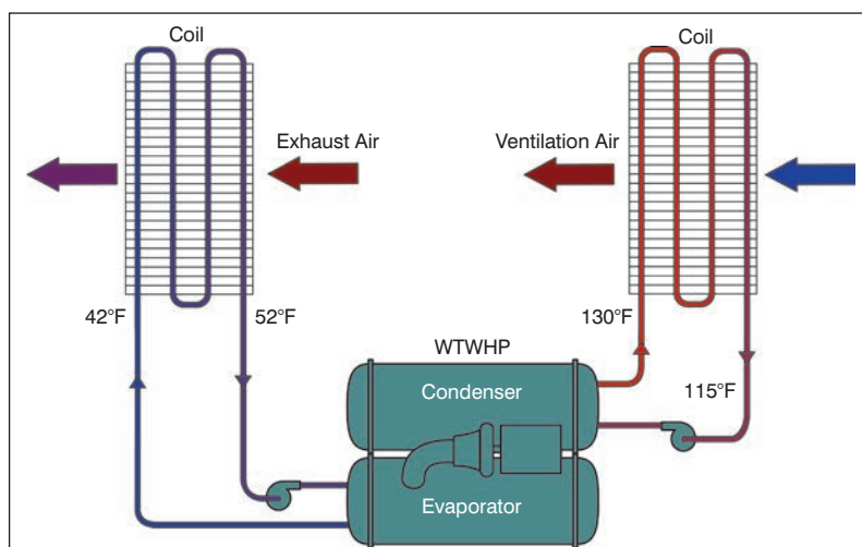
Figure 3: Heat pump system for exhaust air heat recovery.
