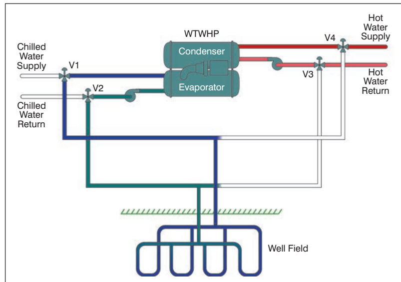
Figure 5: Geothermal system for simultaneous heating and cooling, operating in heating-only mode.
