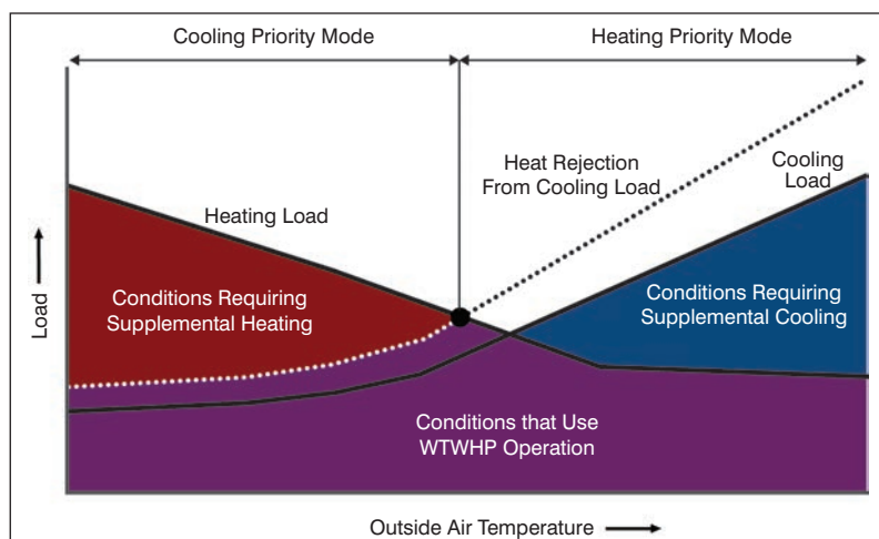
Figure 2: Operating areas for simultaneous heating-and-cooling heat pump.
